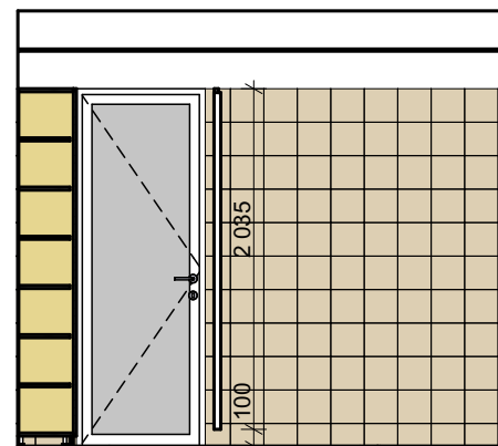
POHLED 2.08_02
