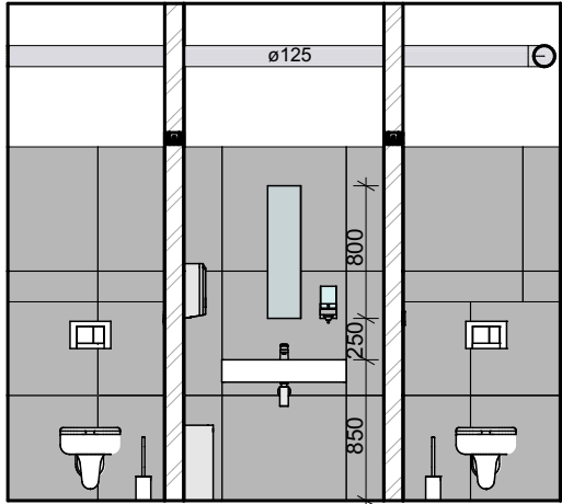
POHLED 1.13_02
