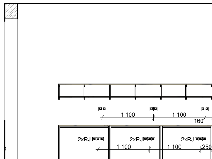
POHLED 2.23_02
