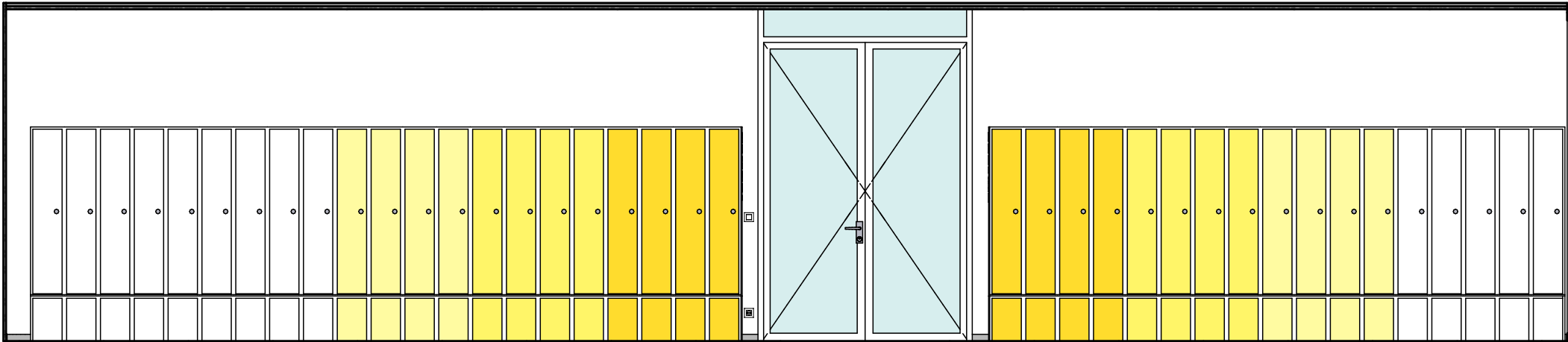
POHLED 1.02_02
