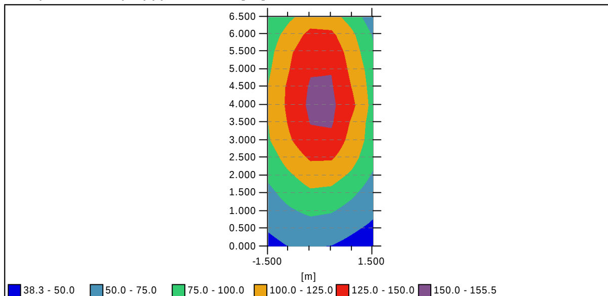
Zona prechazeni, Eh(0 m) (1) : Illuminance [lux]
